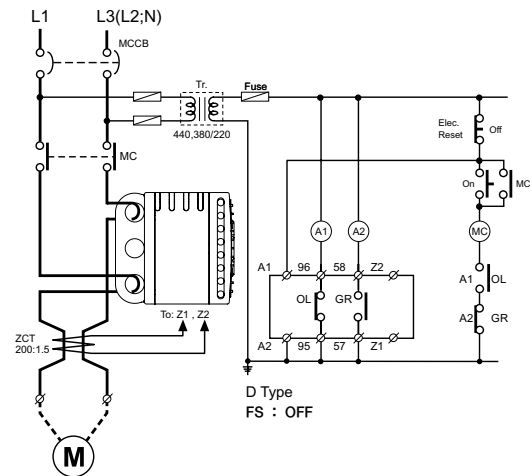
Single phase motor (D type)
