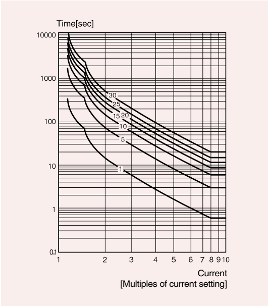
Thermal inverse characteristic
