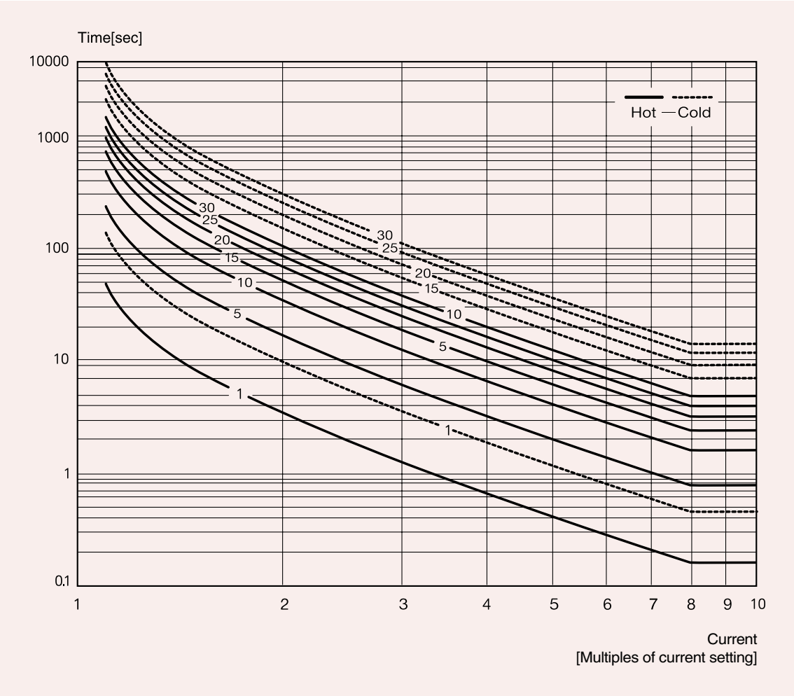
Inverse characteristic
