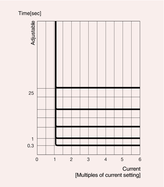
Definite characteristic
